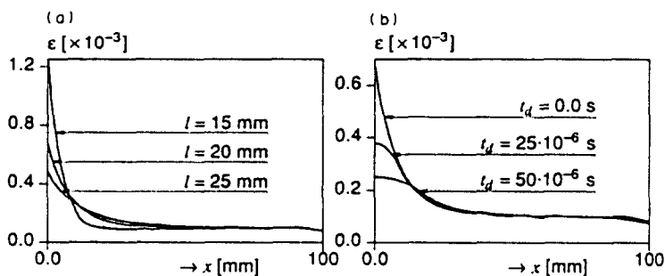
Fig. 8. (a) Variation of the length scale parameter ( t = 0.2 \cdot 10^{-1} s). (b) Variation of the loading rate ( t = 0.2 \cdot 10^{-1} s).
