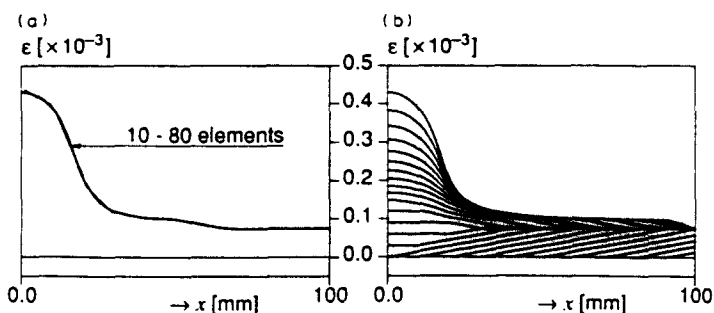
Fig. 7. Rate-dependent model with t_d = 50 \cdot 10^{-6} s. (a) Strain localization along the bar at t = 0.25 \cdot 10^{-1} s. (b) Development of the localization band (80 elements).
